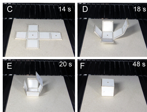
Fig. 7. Fabrication and self-folding of a 20 mm long cube structure with uniform heating. A) Cross-section schematic of the self-folding mechanism. B) bottom, middle, and top layers of the self-folding composite. The bottom and top layers are 0.5 mm thick paperboard, middle layer is 0.5 mm thick pre-strained polystyrene SMP. The three layers are stacked and adhered together with silicone adhesive film. C-F) Frames from a self-folding experiment in which the laminate was introduced into an oven preheated to 170°C. Also indicated are the time of each frame from the beginning of the experiment.
