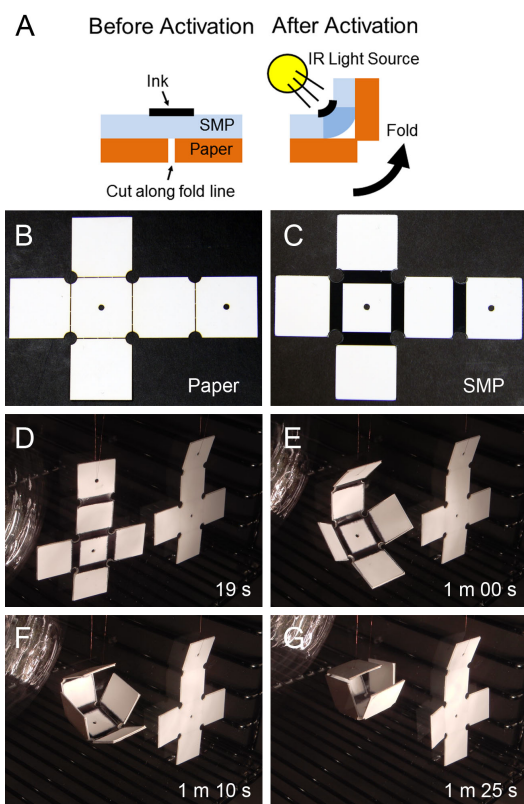
Fig. 1. Light activated self folding of a 20 mm long cube. A) Cross section schematic of light activated folding. B) Paperboard and C) SMP layers compose a two-piece laminate. Black lines of ink are printed directly onto the SMP prior to laser machining. D-G) Frames from experiment in which two laminates, one with ink and one without, were introduced into an oven preheated to 90°C. An infrared light was shone through the front glass of the oven. The printed black lines absorb enough light energy to locally activate the SMP.
